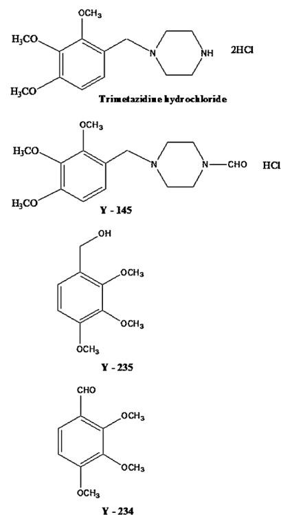
Figure 1. Structures of trimetazidine dihydrochloride and its impurities (Y-145, Y-234, and Y-235)
